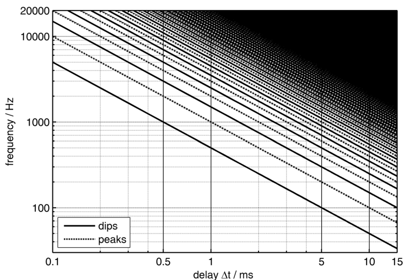
Figure 2: Position of peaks and dips in a comb-filter-shaped transfer function for different delay times \Delta t
