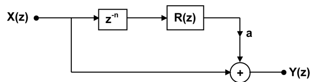
Figure 1: Audio system with a comb-filter-shaped transfer function
