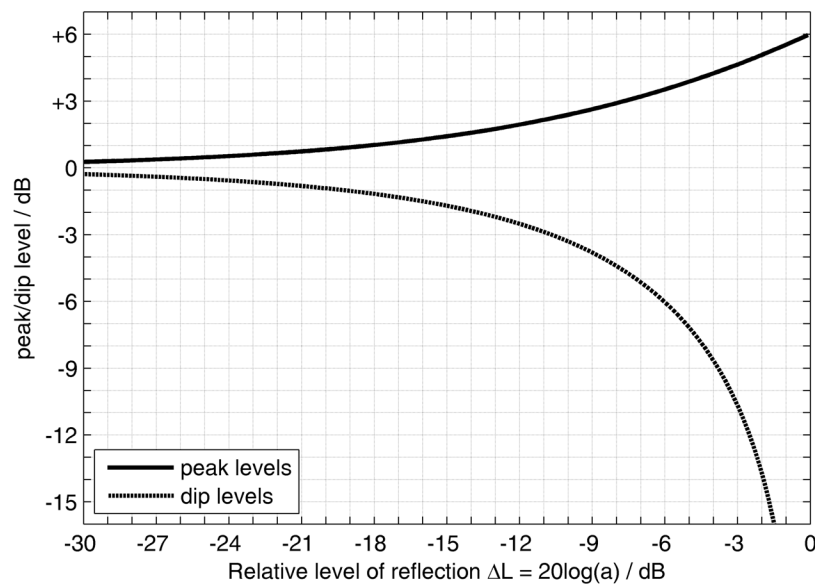
Figure 3: Altitude of peaks and dips in the comb-filter-shaped transfer function due to reflections with relative level \Delta L
