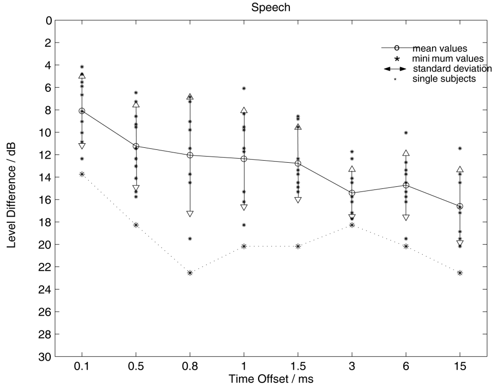
Figure 5: Just noticeable difference between original and comb-filtered signal showing the level difference between direct and delayed signal for delay times (time offsets) between 0.1 and 15 ms.
